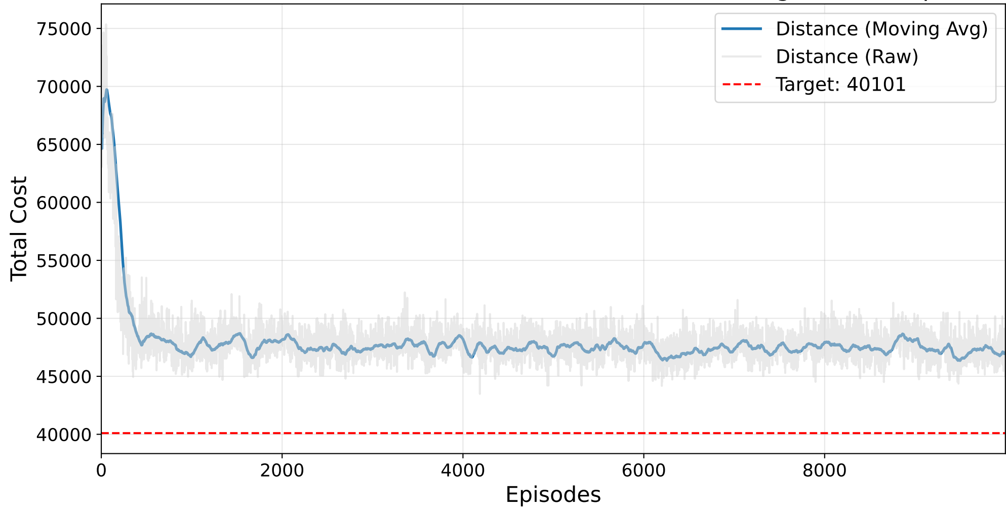
Final HYPERBAND TPE Masked AutoRL-SOP Training - ft70.2.sop
